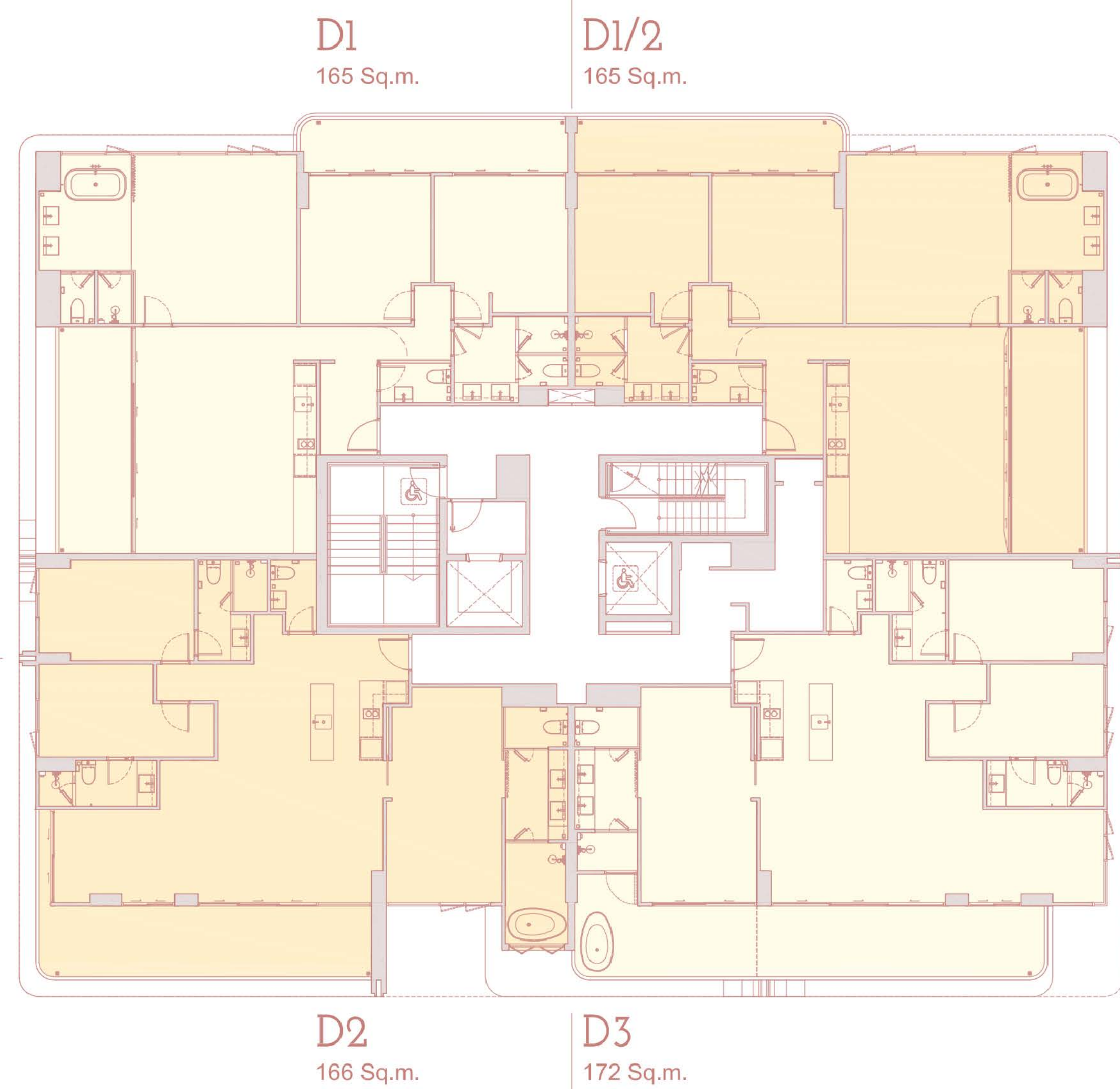
7th Floor Plan 1 5 10
